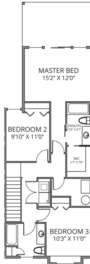
SECOND FLOOR PLAN 904 SQ. FT.
