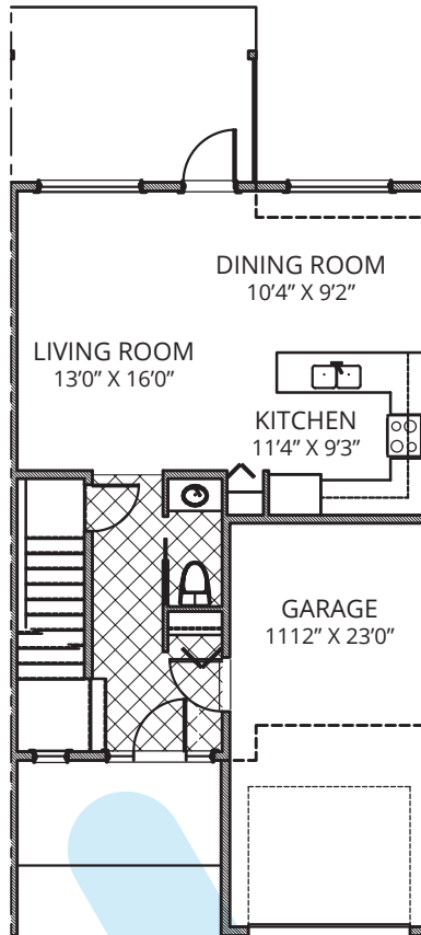
GROUND FLOOR PLAN 624 SQ. FT.
